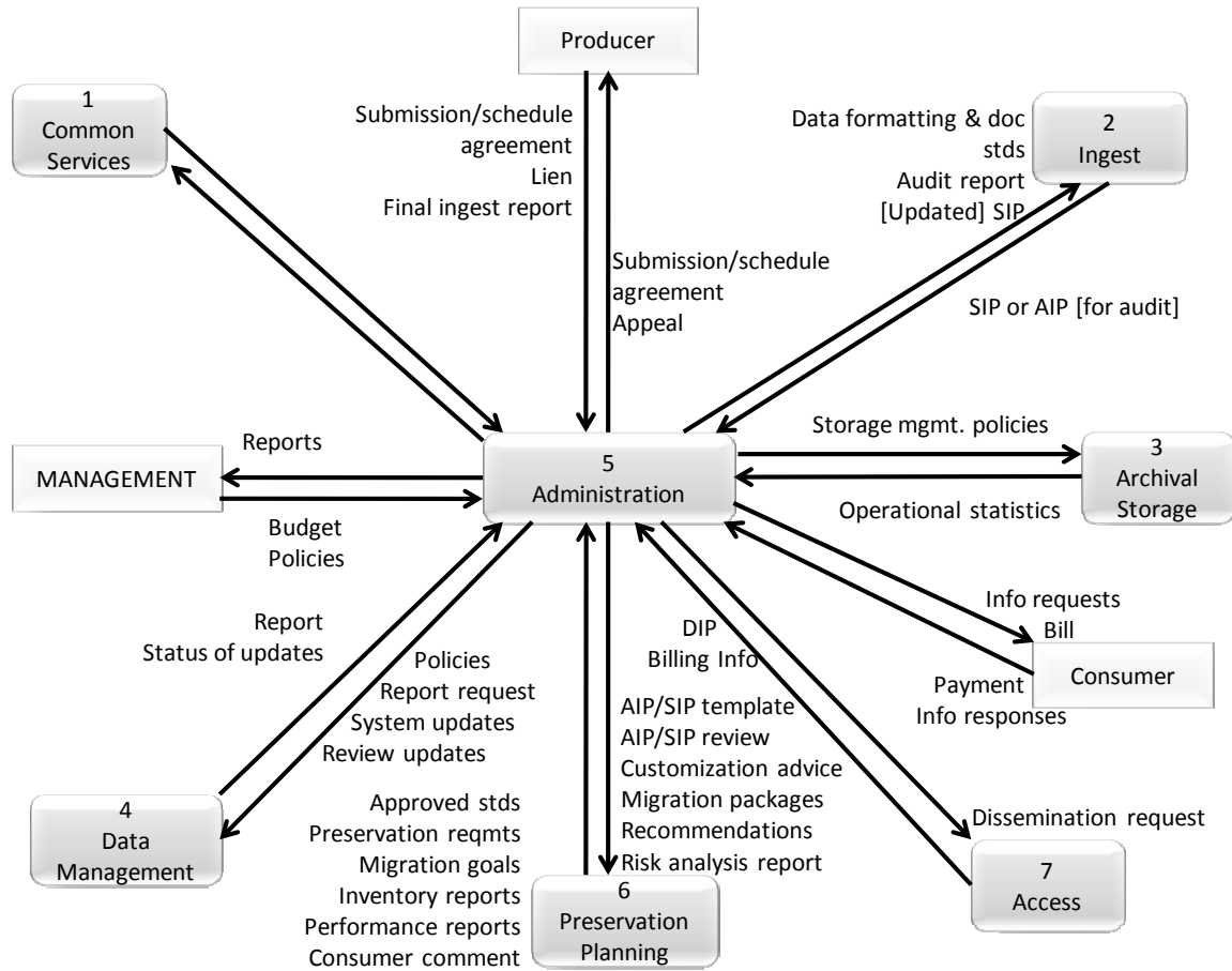
Figure 4-9: Administration Context Diagram
